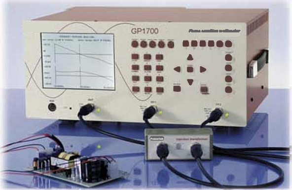
GP1700 with Powertek injection transformer testing an SMPS
